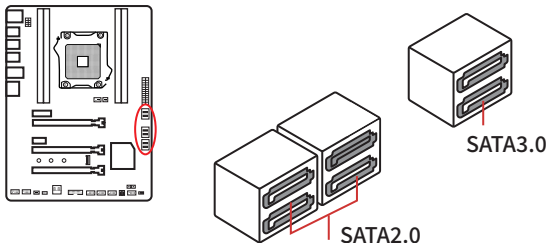
2-11 SATA Interface
