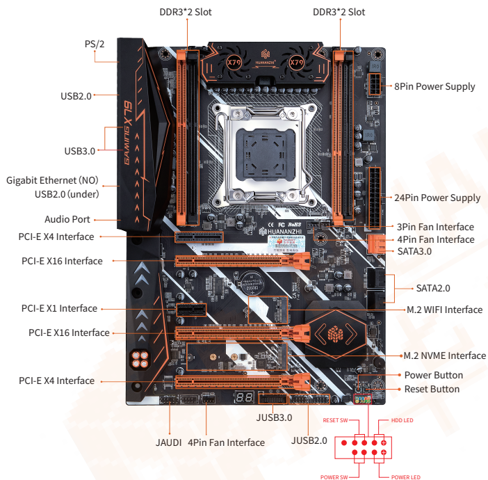
1-1 X79 Deluxe V7.1 Motherboard Illustration
